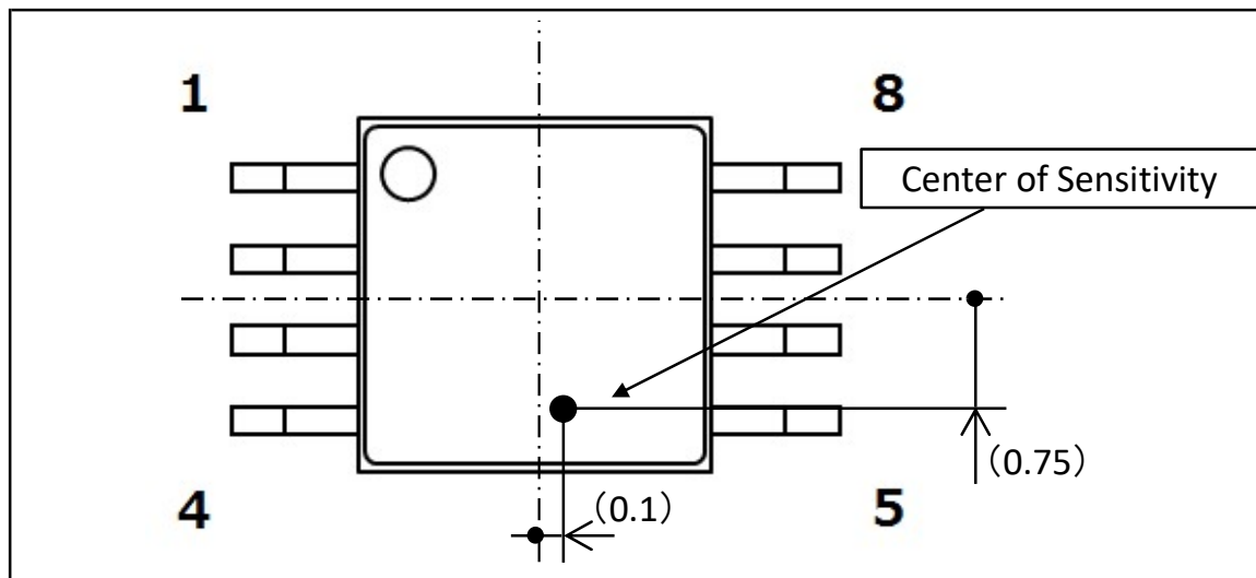
Figure 2-1 Pin Configuration
