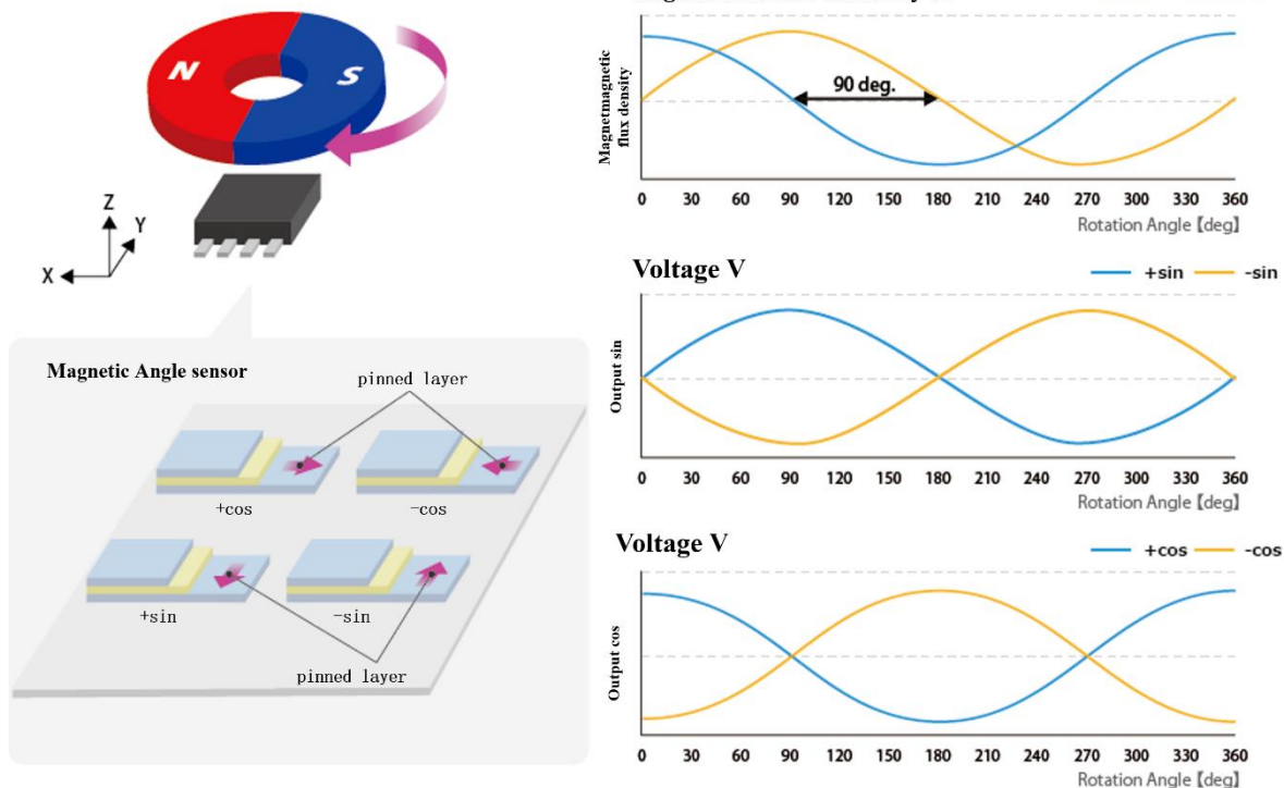
Fig.1 Output signal of magnetic angle sensor
