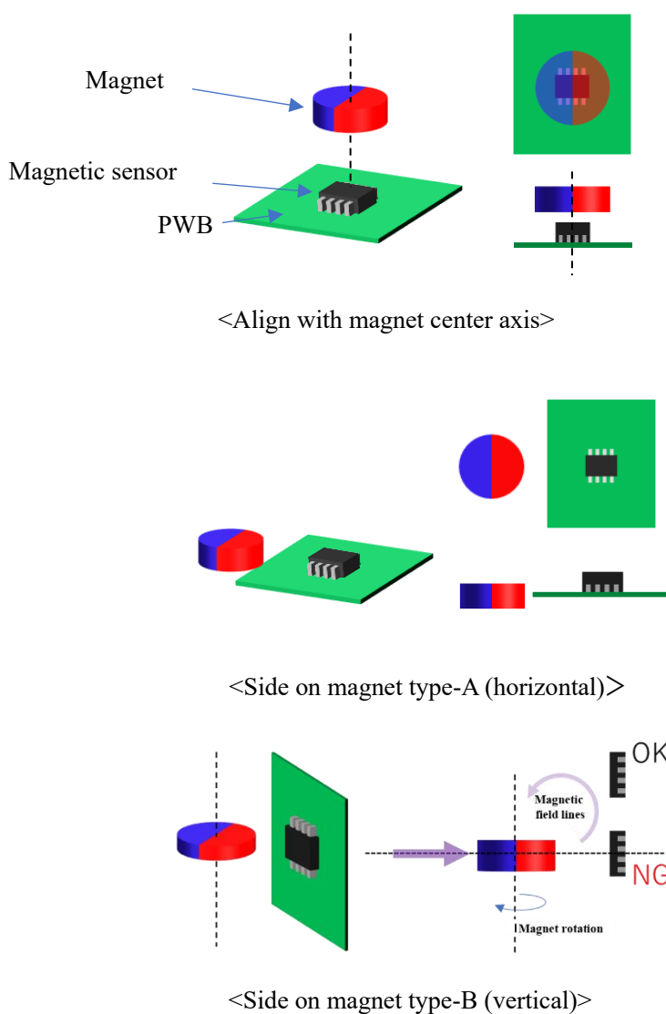
Fig.5 Layout of magnetic angle sensor
