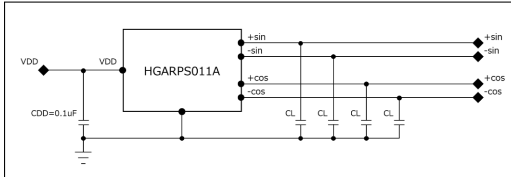
Fig.7 Reference circuit for magnetic angle sensor
