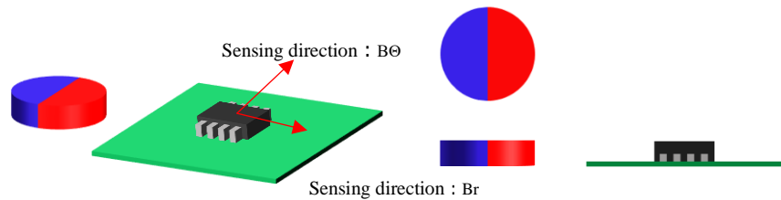
Fig.13 Layout of the magnet
