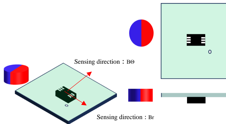
Fig.13 Layout of the magnet
