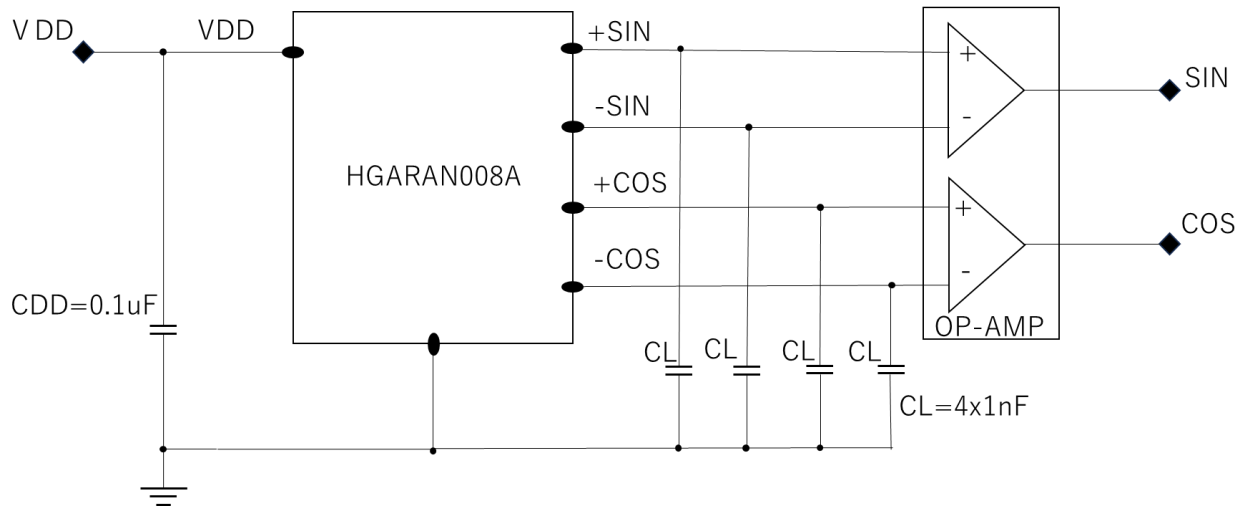
Fig.7 Reference circuit for magnetic angle sensor
