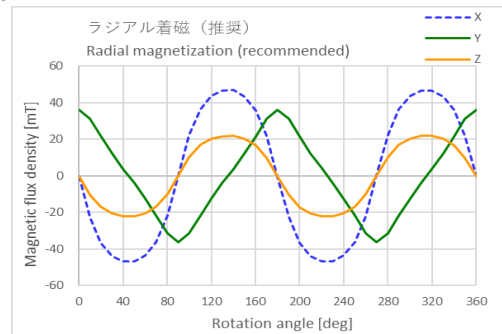
z方向磁場成分 Z-direction magnetic field composition
