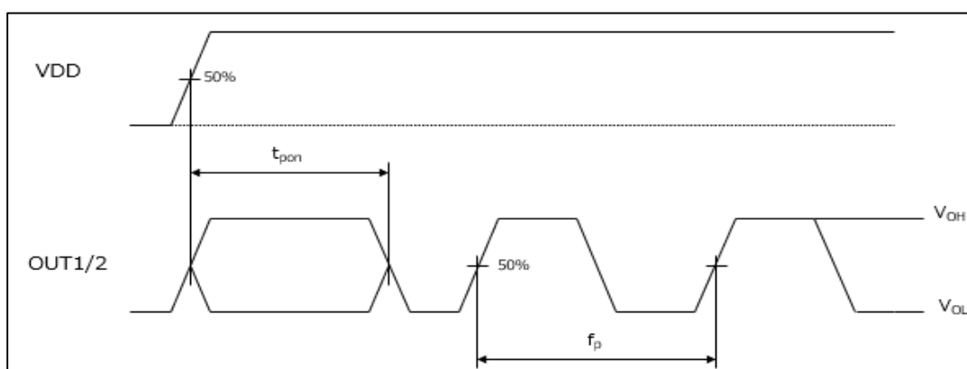
Figure 3-4 Timing Chart
