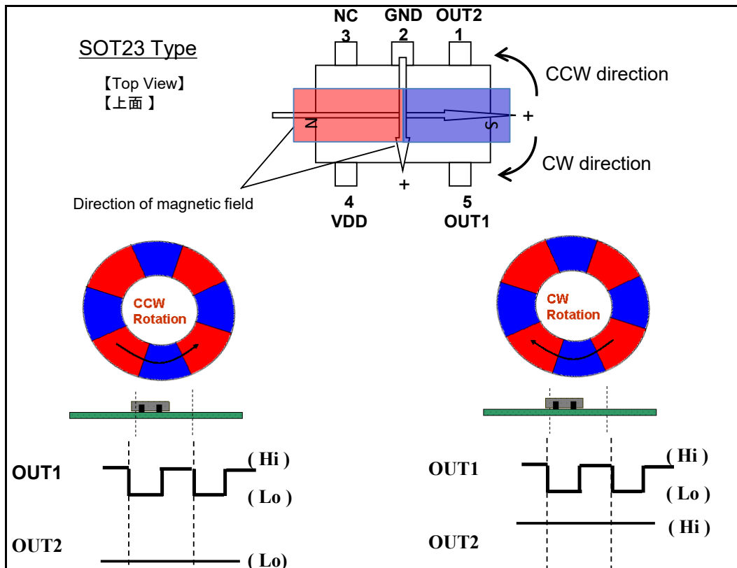
Figure 3-3 Magnetic characteristics:at multi-pole magnet rotation
