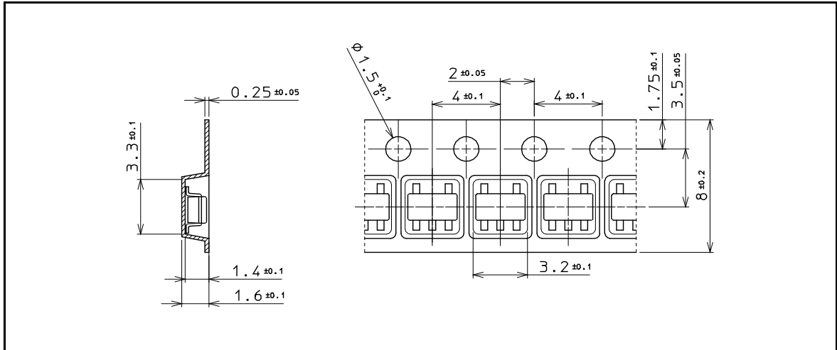
Figure 5-1 Packing of the HGPRDT006A in a tape
