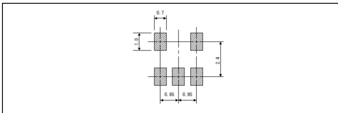
Figure 4-2 Footprint
