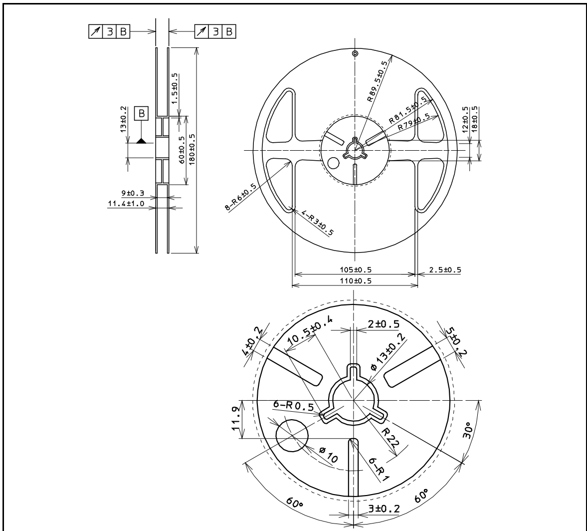
Figure 5-2 Reel Dimensions
