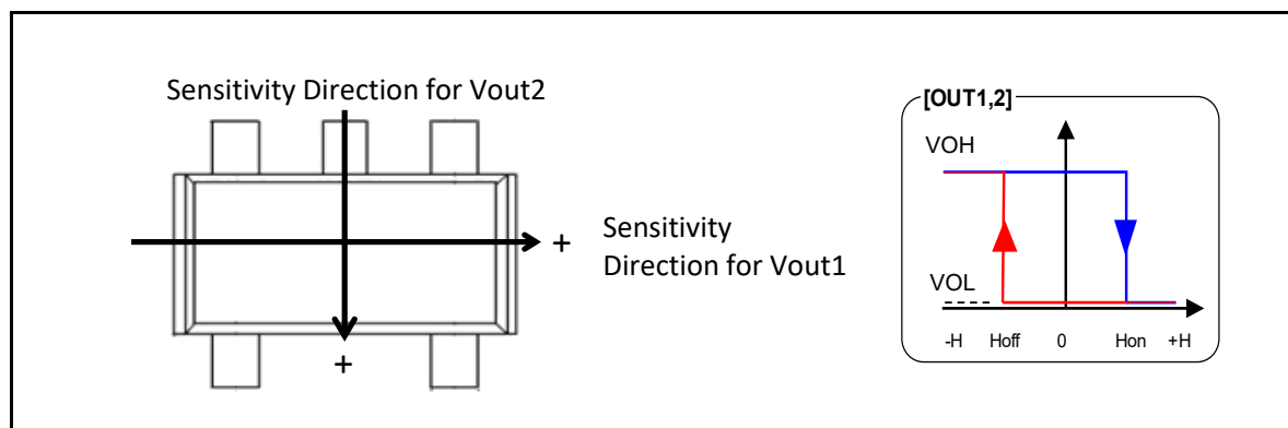
Figure 3-5 Definition of Sensitivity Direction
