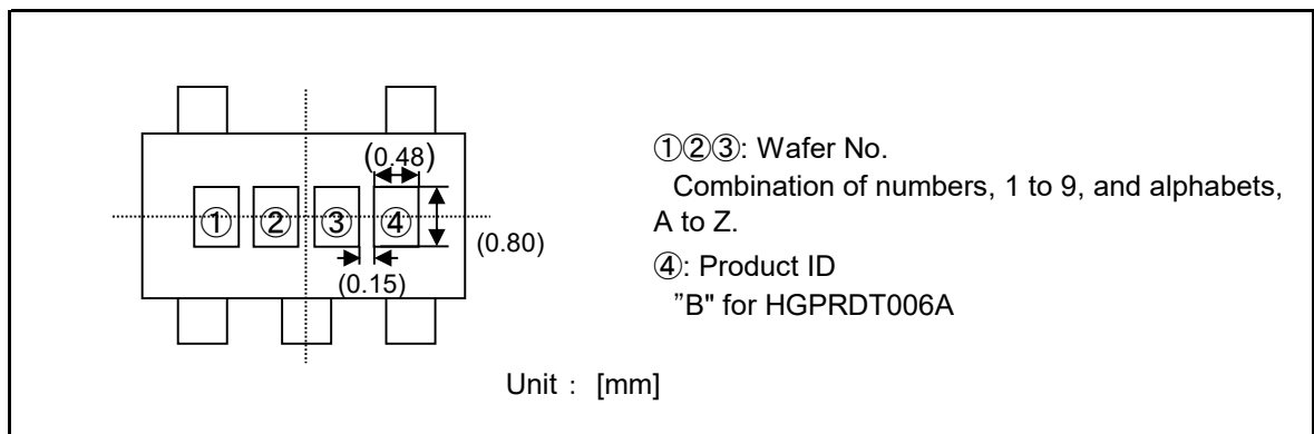
Figure 4-4 Marking of HGPRDT006A
