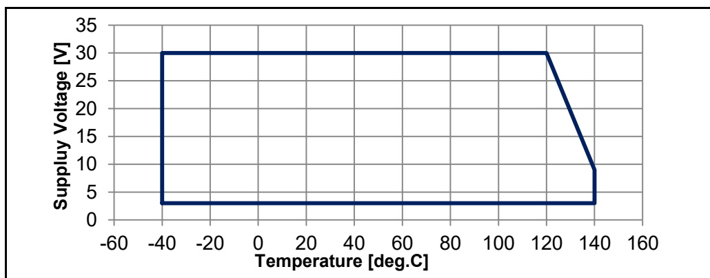
Figure 3-2 Operating Range about Supply Voltage and Temperature
