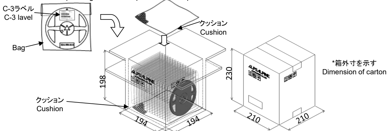
Figure 5-4 Packing for Overseas
