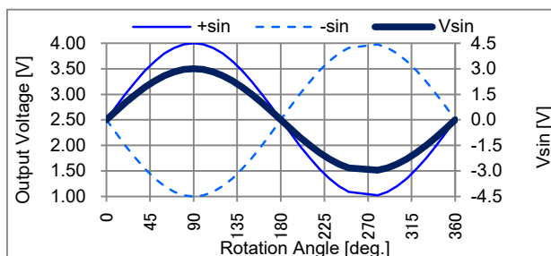
a) Definition of Vsin
