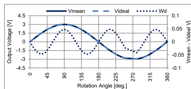
d) Definition of Wd
