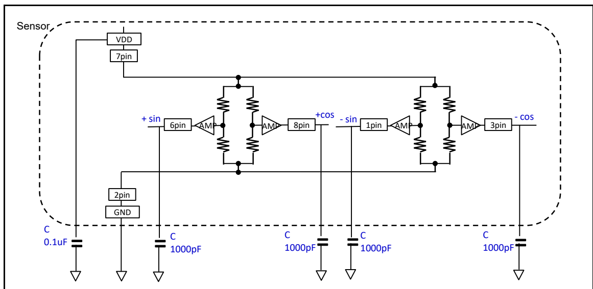
Figure 3-2 Equivalent Circuit & By-pass capacitance recommendation
