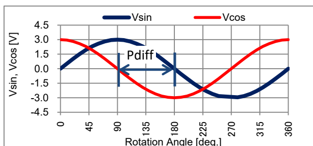
c) Definition of Pdiff
