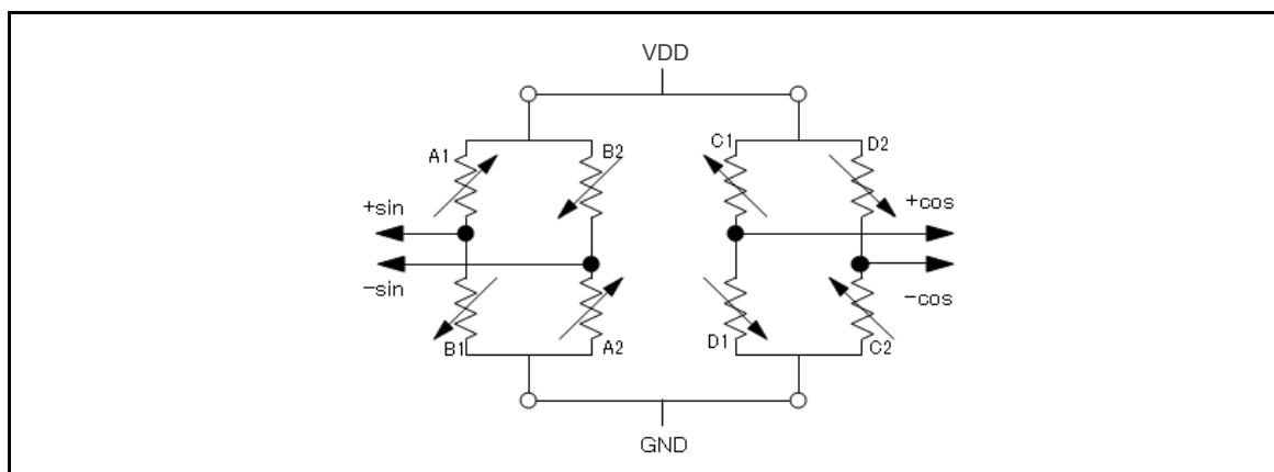
Figure 3-2 Equivalent Circuit
