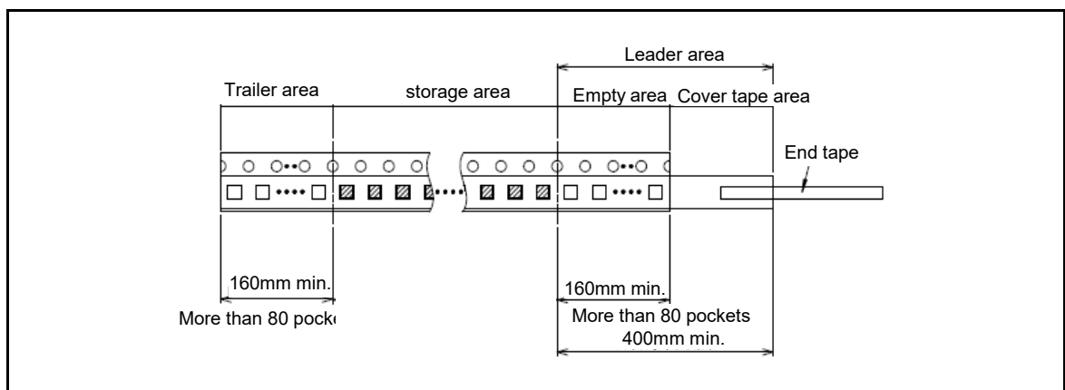
Figure 5-5 Taping Specification
