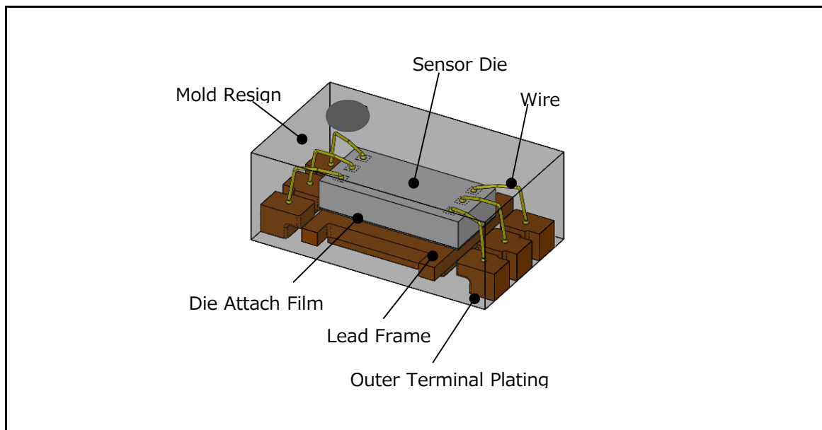
Figure 4-4 Internal Structure
