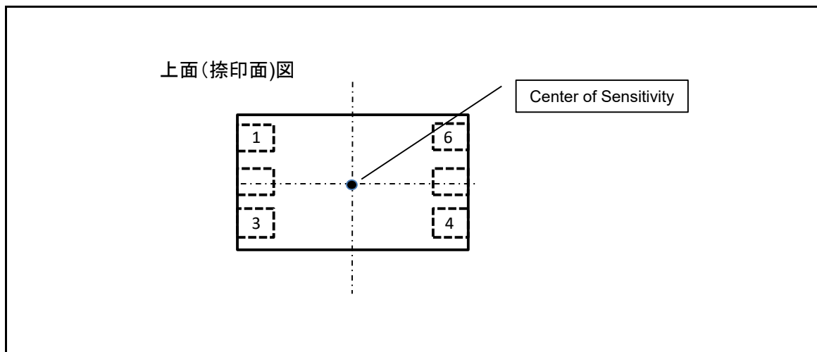
Figure 2-1 Pin Configuration
