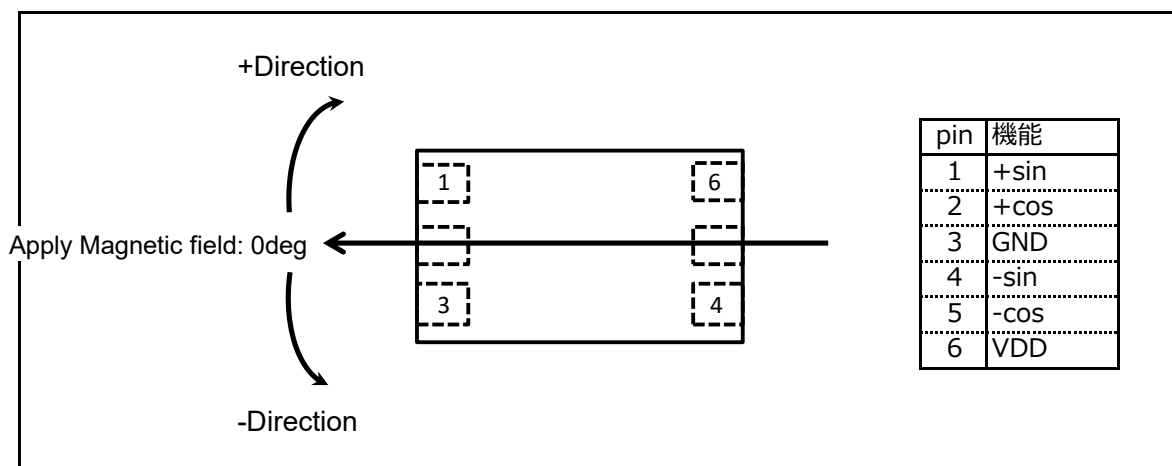
Figure 3-1 Definition of Magnetic Field Direction
